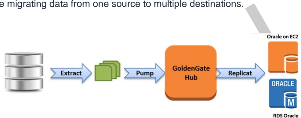
Oracle GoldenGate replication data flow process
