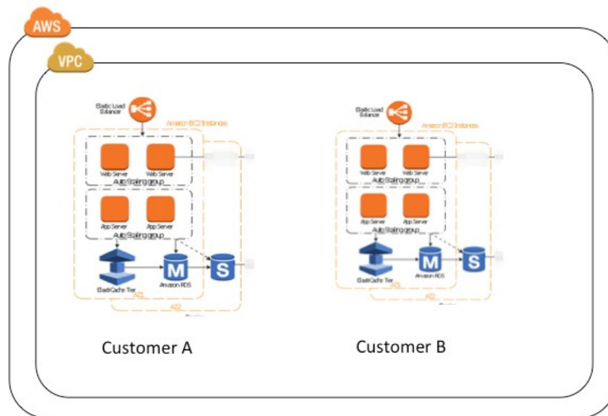
Figure 10: Tenant isolation at VPC subnet layer
