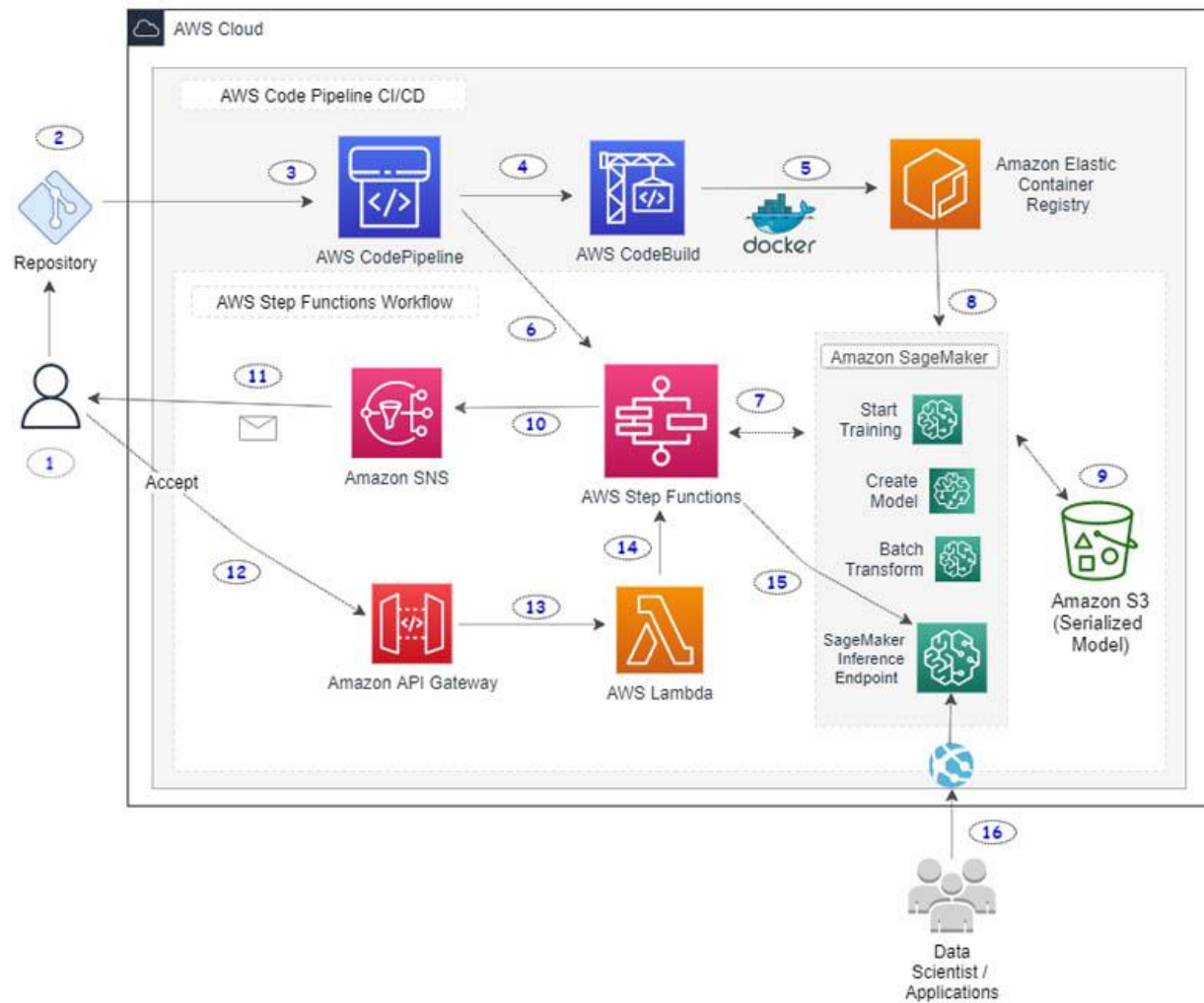
ml-best-practices-public-sector-organizations/ml-best-practices-public-sector-organizations.html Figure 3: Reference Architecture CI/CD Pipeline for ML on AWS
