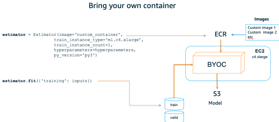
Figure 2: Bring your own container
