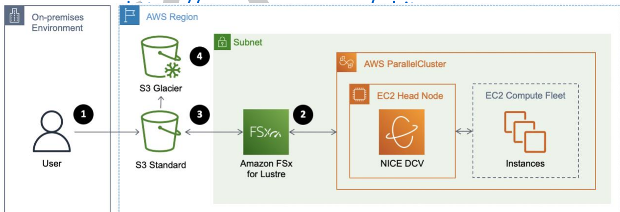
Figure 7: Data lifecycle
