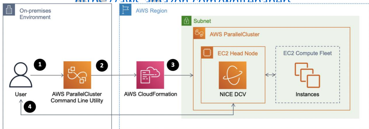
Figure 3: Example AWS ParallelCluster architecture
