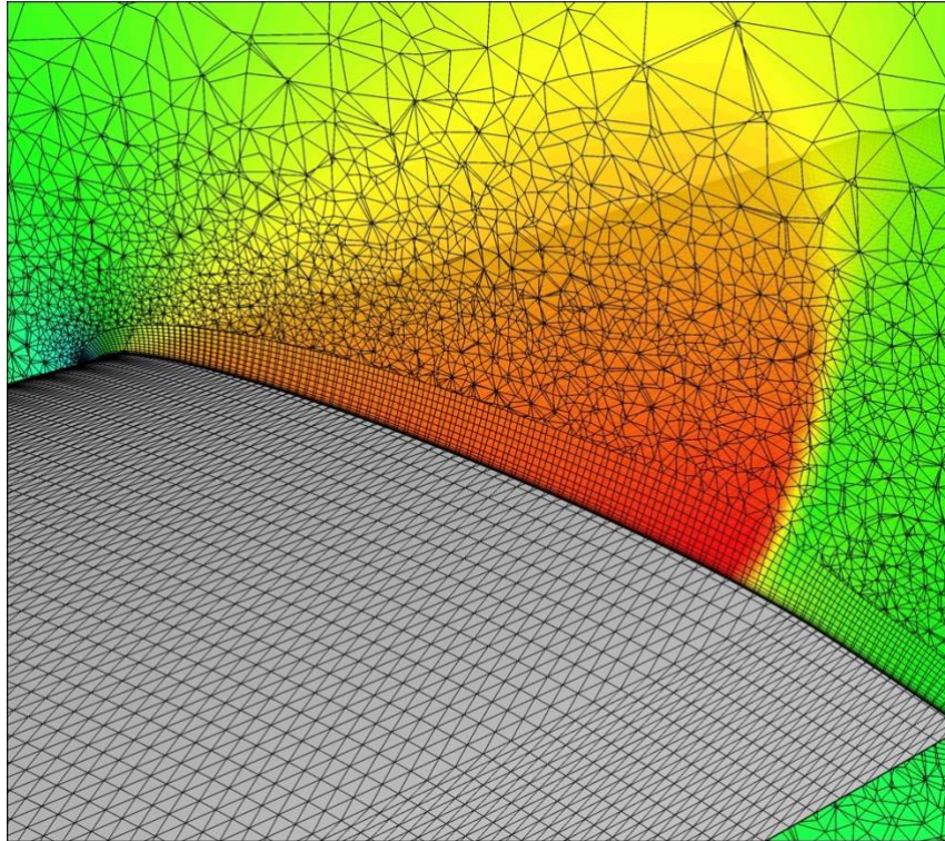
Figure 1: Mesh generation
