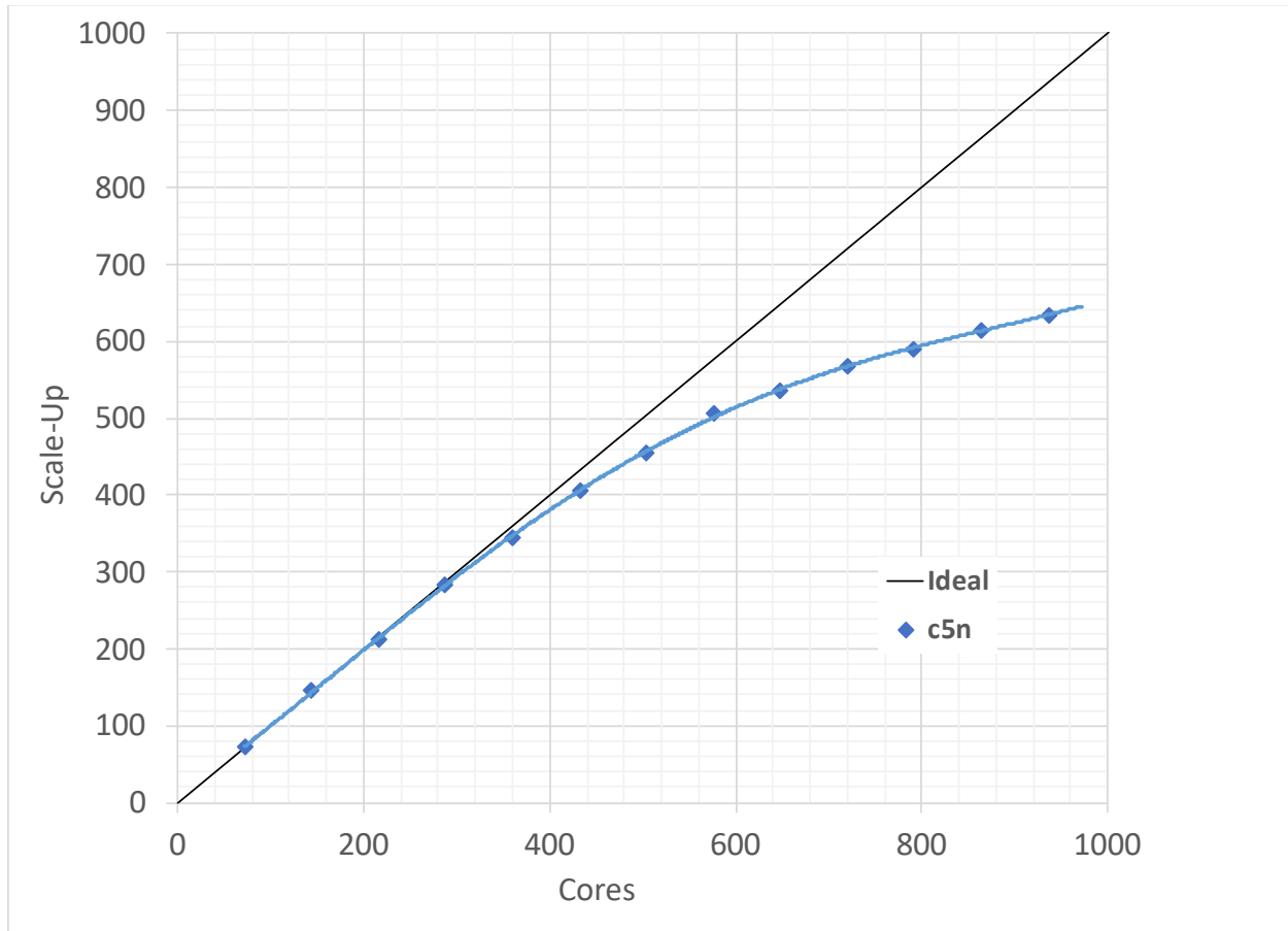
For the latest technical content, refer to the AWS Whitepapers & Guides page: Figure 4. Strong scaling demonstrated for a 14M cell external aerodynamics use case
