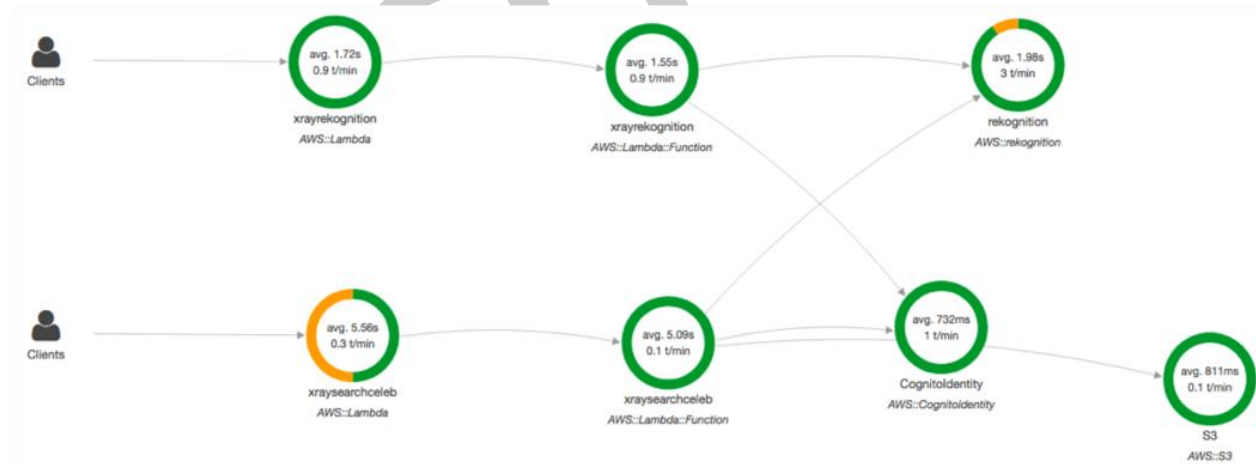
Figure 7: AWS X-Ray Service Map visualizing 2 services
