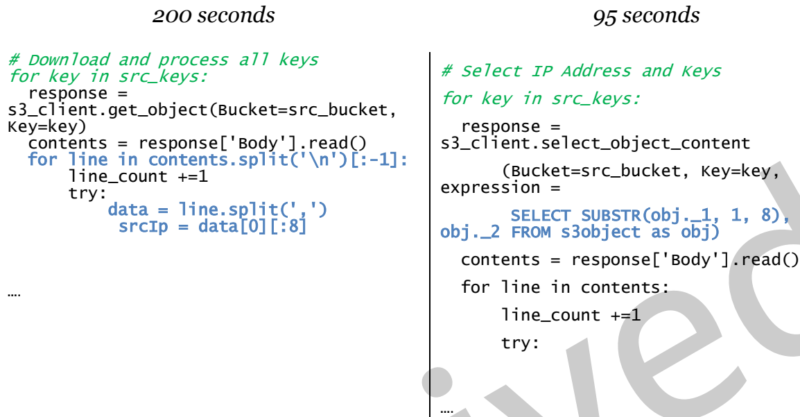
Figure 18: Lambda performance statistics using Amazon S3 vs S3 Select
