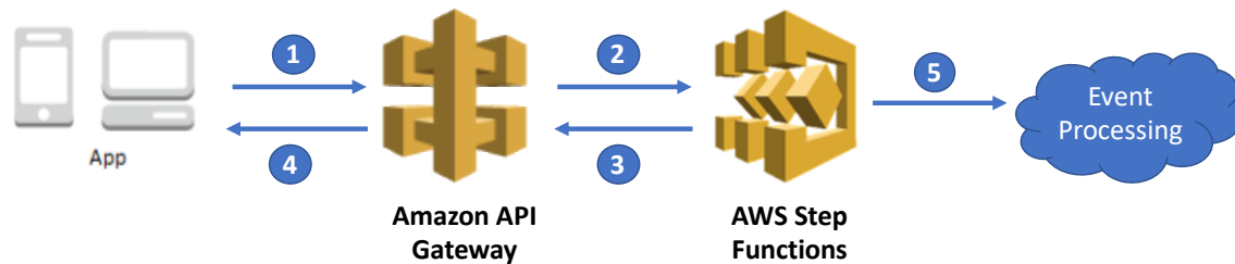
Figure 24: Asynchronous workflow with Step Functions state machines
