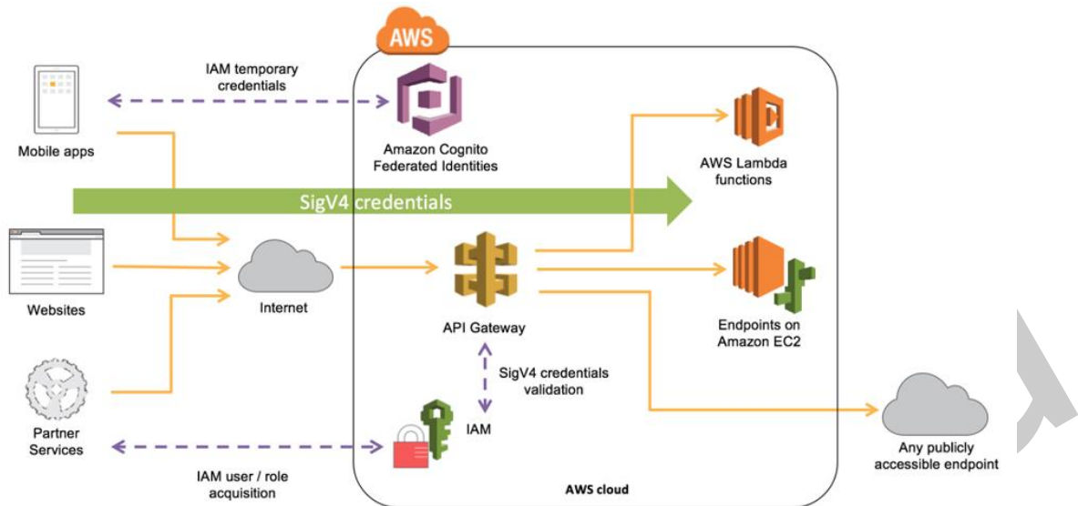
Figure 10: AWS_IAM authorization
