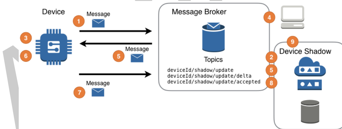
Figure 4: Using Device Shadow with devices.
