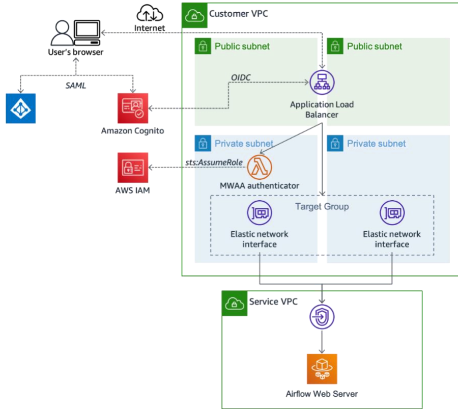
Figure 1 – Architecture overview
