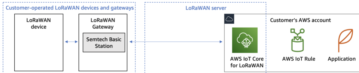
AWS IoT Core for LoRaWAN architecture
