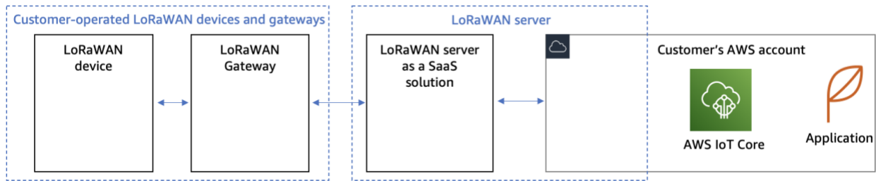
LoRaWAN server provided and operated by an AWS Partner
