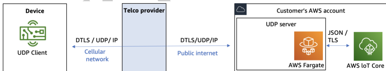
Architecture of a customer-operated solution secured by DTLS
