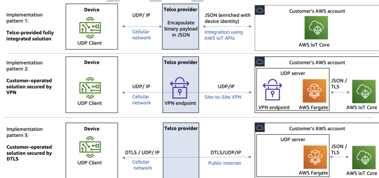
Patterns for implementing IoT solutions with AWS using UDP protocol
