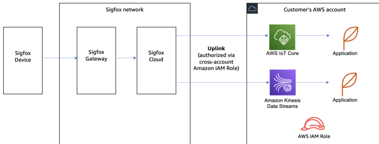
Example architecture for processing uplink data from Sigfox devices
