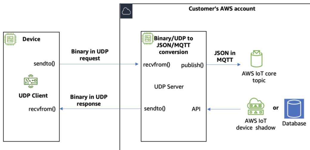
Example architecture for processing UDP datagrams with AWS
