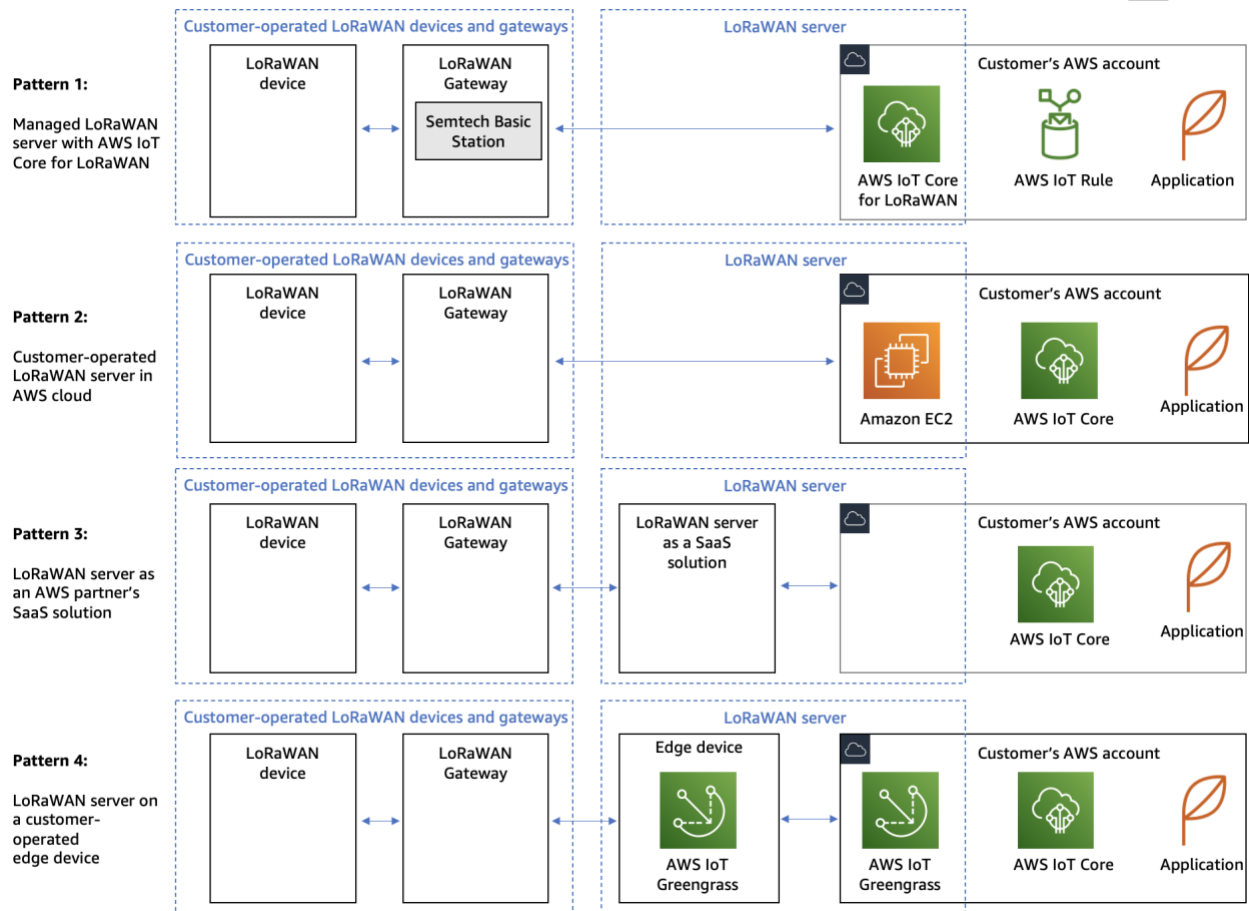
Patterns for deployment of private LoRaWAN networks
