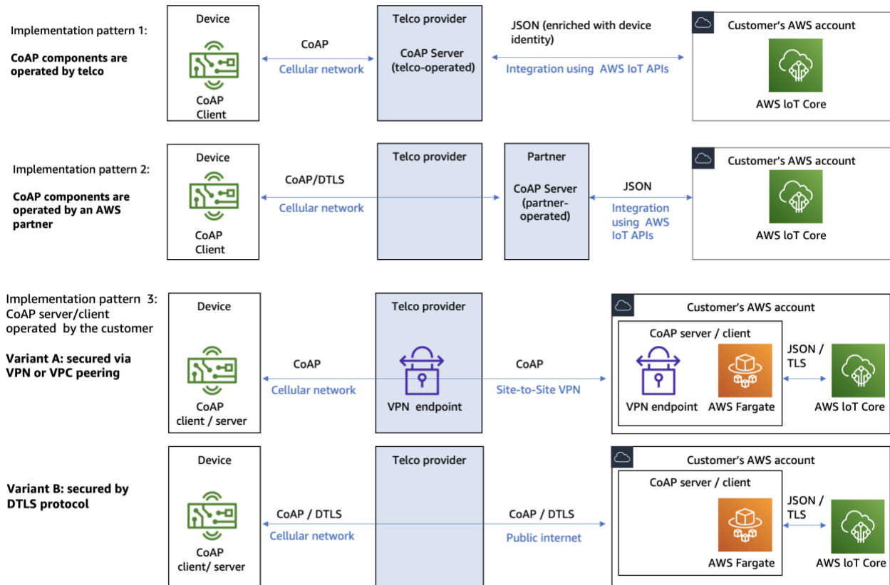
Patterns for implementing IoT solutions with AWS using CoAP
