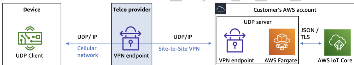
Architecture of a customer-operated solution secured by VPN
