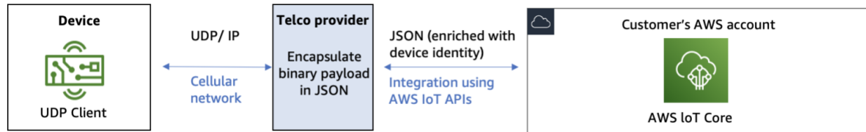
Architecture of a fully integrated solution provided by the telco
