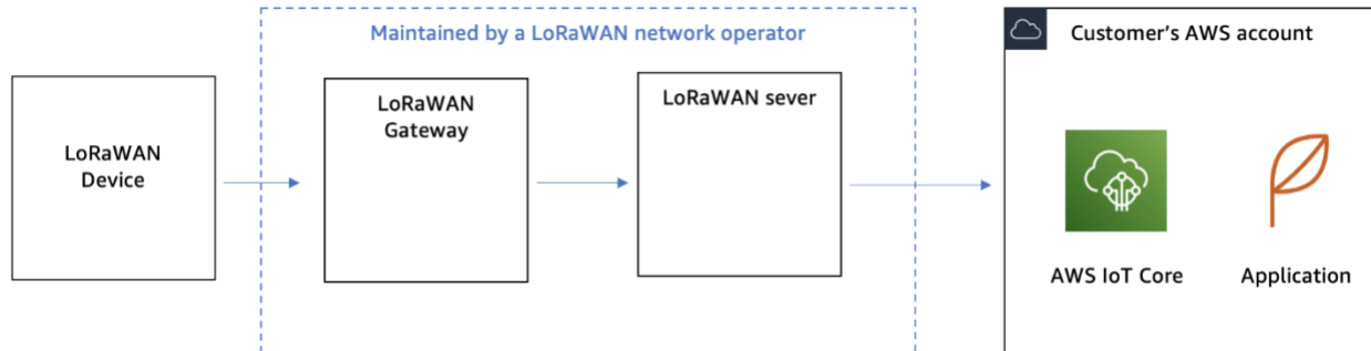
Example architecture for using a public LoRaWAN network with AWS
