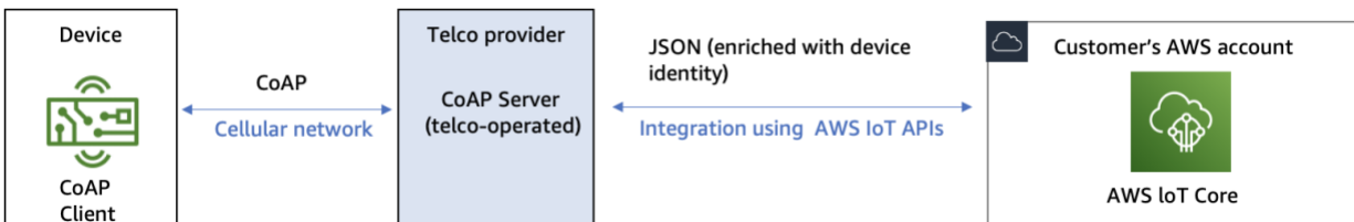
Architecture for CoAP server operated by telco
