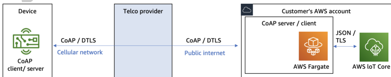
Using DTLS to secure data in transit
