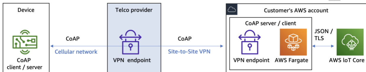
Using VPN to secure data in transit
