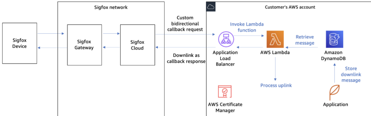
Example architecture for sending downlink data to Sigfox devices
