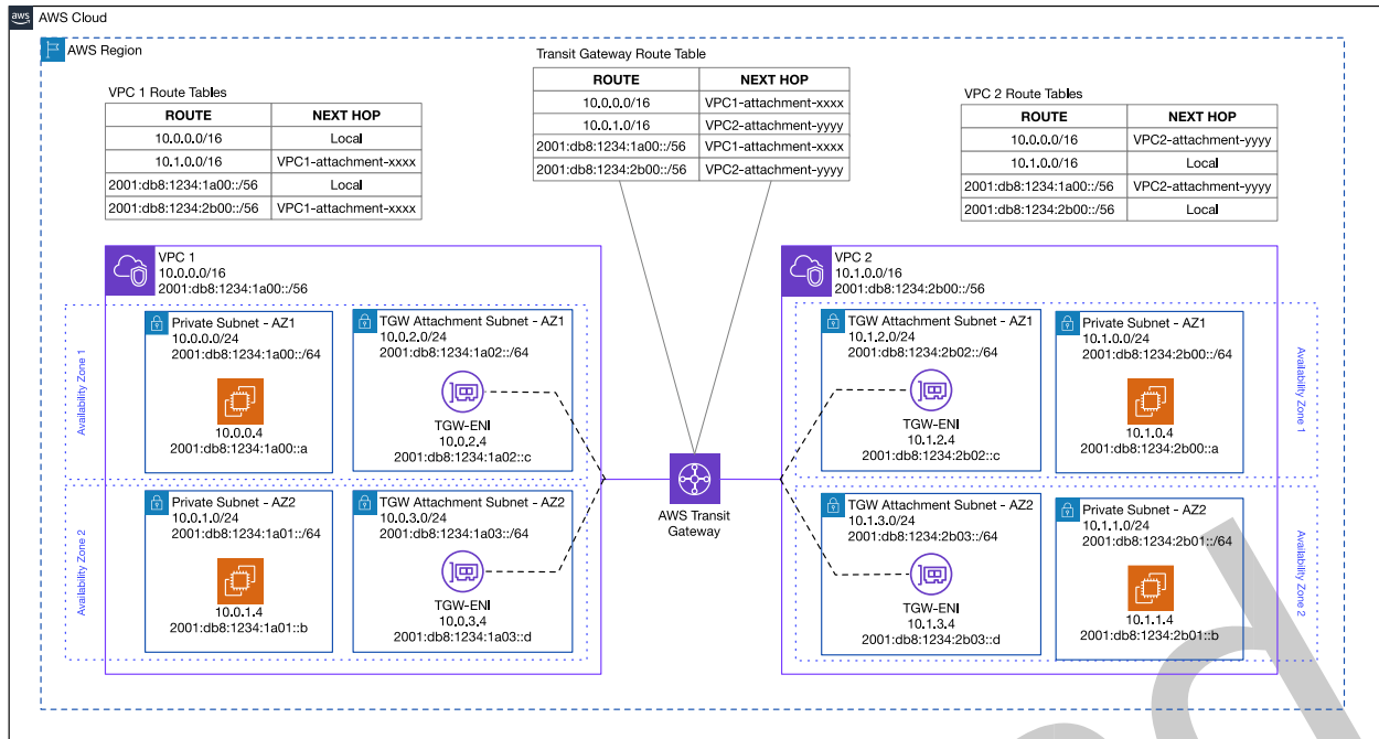
Dual-stack AWS Transit Gateway routing
