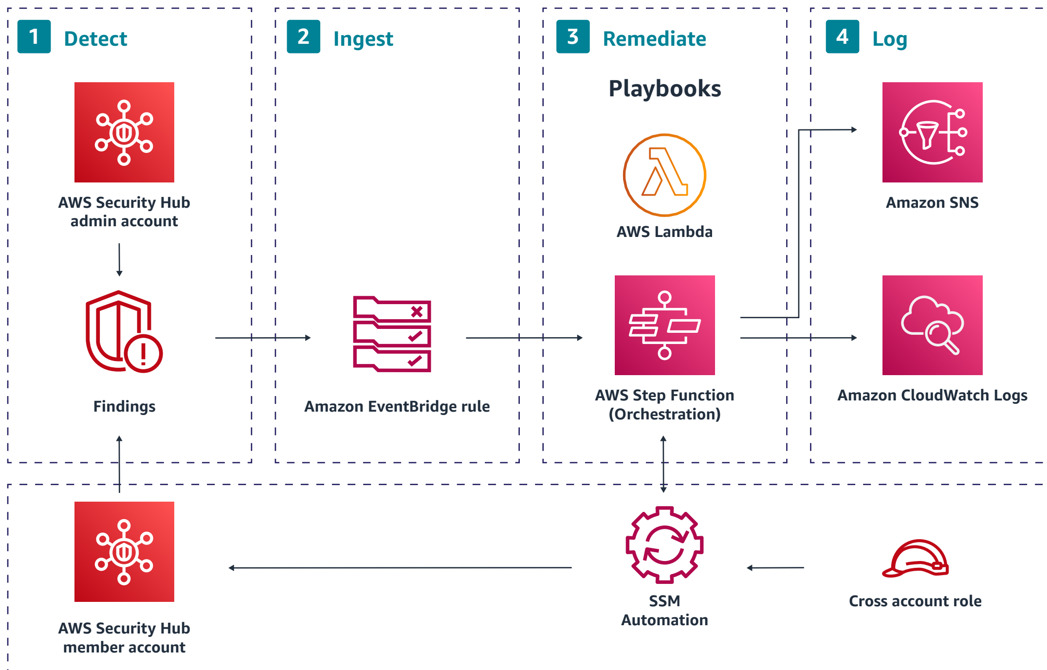
Figure 6 – Security Hub Automated Response and Remediation
