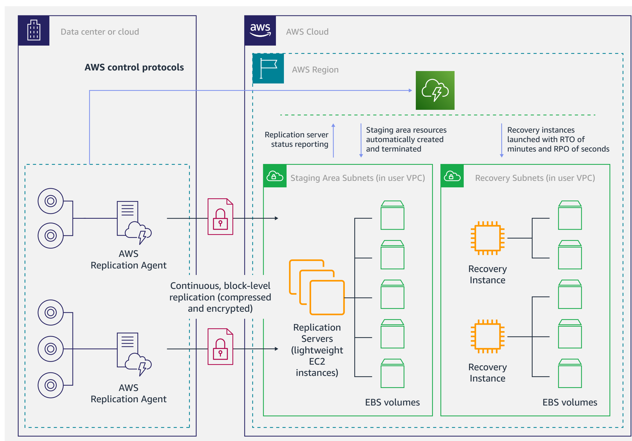
Figure 7 – AWS Elastic Disaster Recovery continuous replication of on-premises and cloud servers
