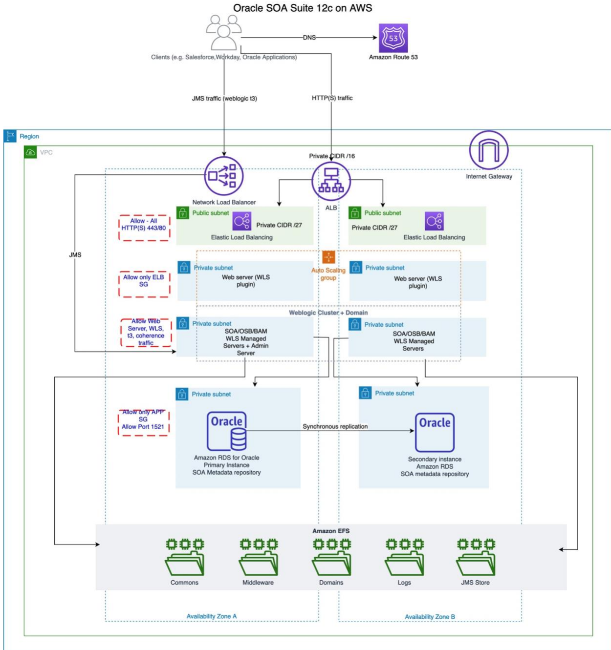
Figure 2: High level architecture of Oracle SOA Suite 12c on AWS
