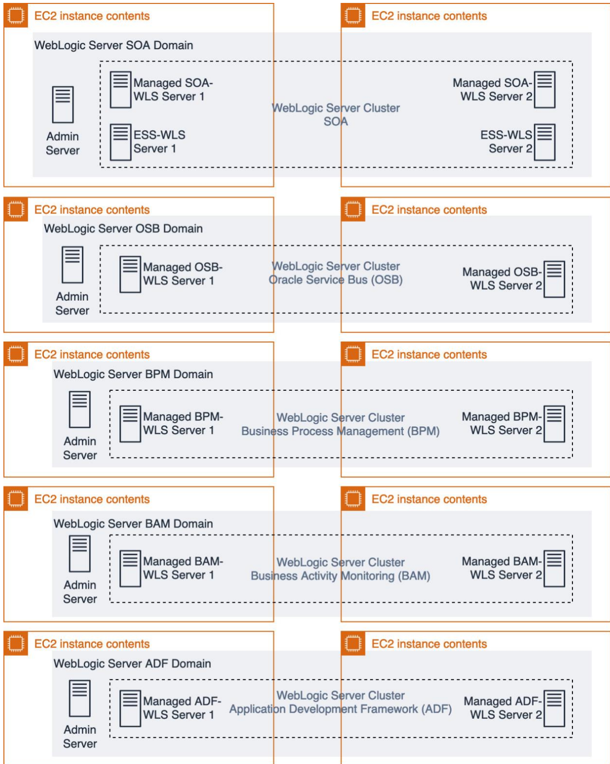
Figure 1: Oracle SOA Suite components deployed on Oracle WebLogic Server
