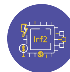
Amazon Inferentia2
