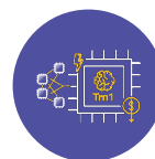
Amazon Trainium
