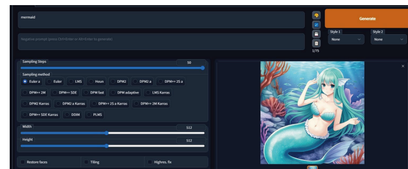
AUTOMATIC1111
