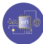
Amazon Inferentia
